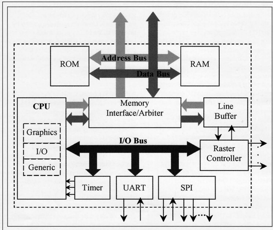
Fig. 4: The Easy GUI™ controller chip is highly integrated, containing the circuitry required to provide the functions of many peripheral devices.
