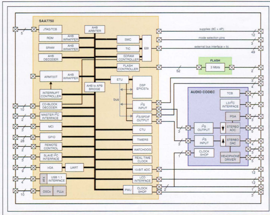
Fig. 5: The second chip in the design is the SAA7750; it incorporates both a microprocessor and an audio codec, as well as flash memory to allow field upgrades to the system software.
