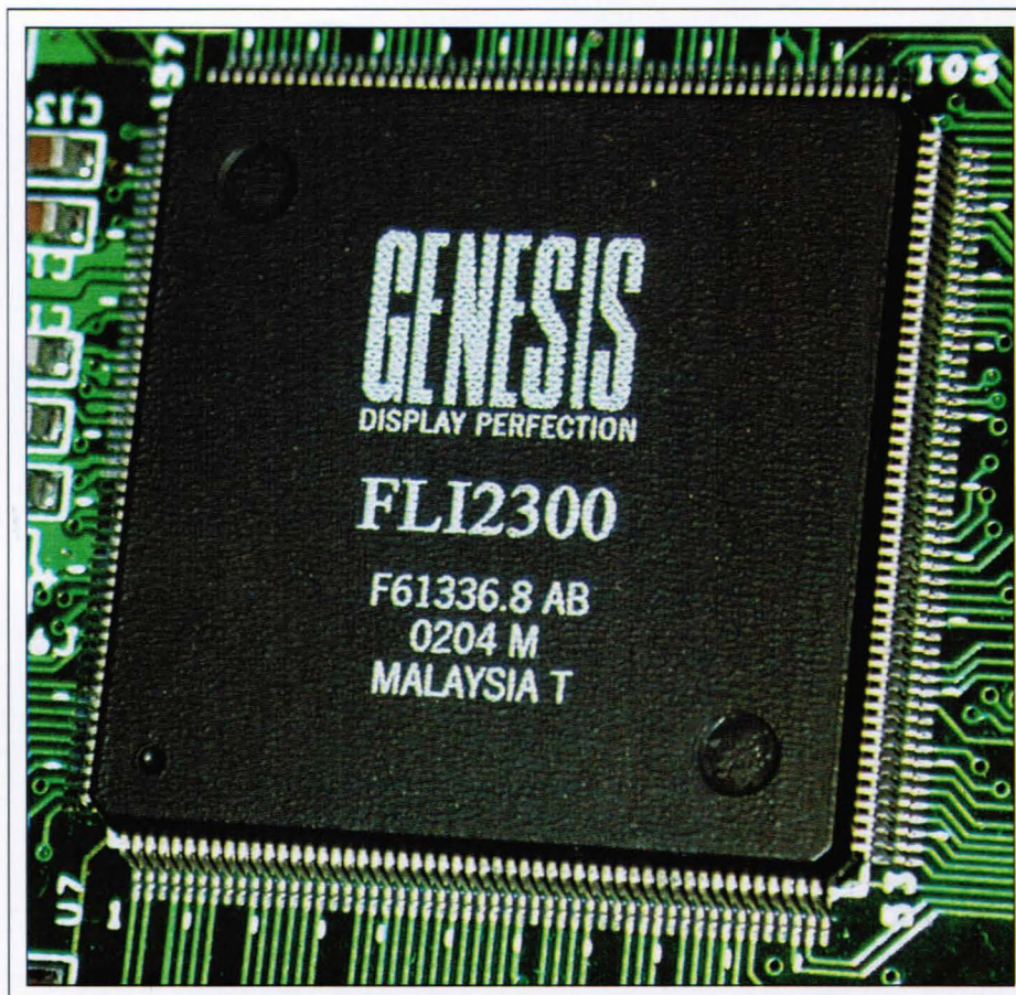
Fig. 2: The FLI2300 chip integrates many video-processing functions, including motion-adaptive de-interlacing with film mode, DCDi™, cross-color suppression, noise reduction, scaling, video enhancement, and frame-rate conversion.
