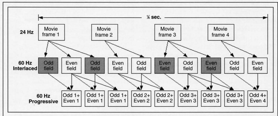
Fig. 2: Images that originated on film and were then converted to video using a teleciné machine are very common. In NTSC, the teleciné process converts the 24-frames/sec film into 60-fields/sec interlaced video using a process known as “3:2 pull-down.” A process called “reverse 3:2 pull-down” is used for de-interlacing.
